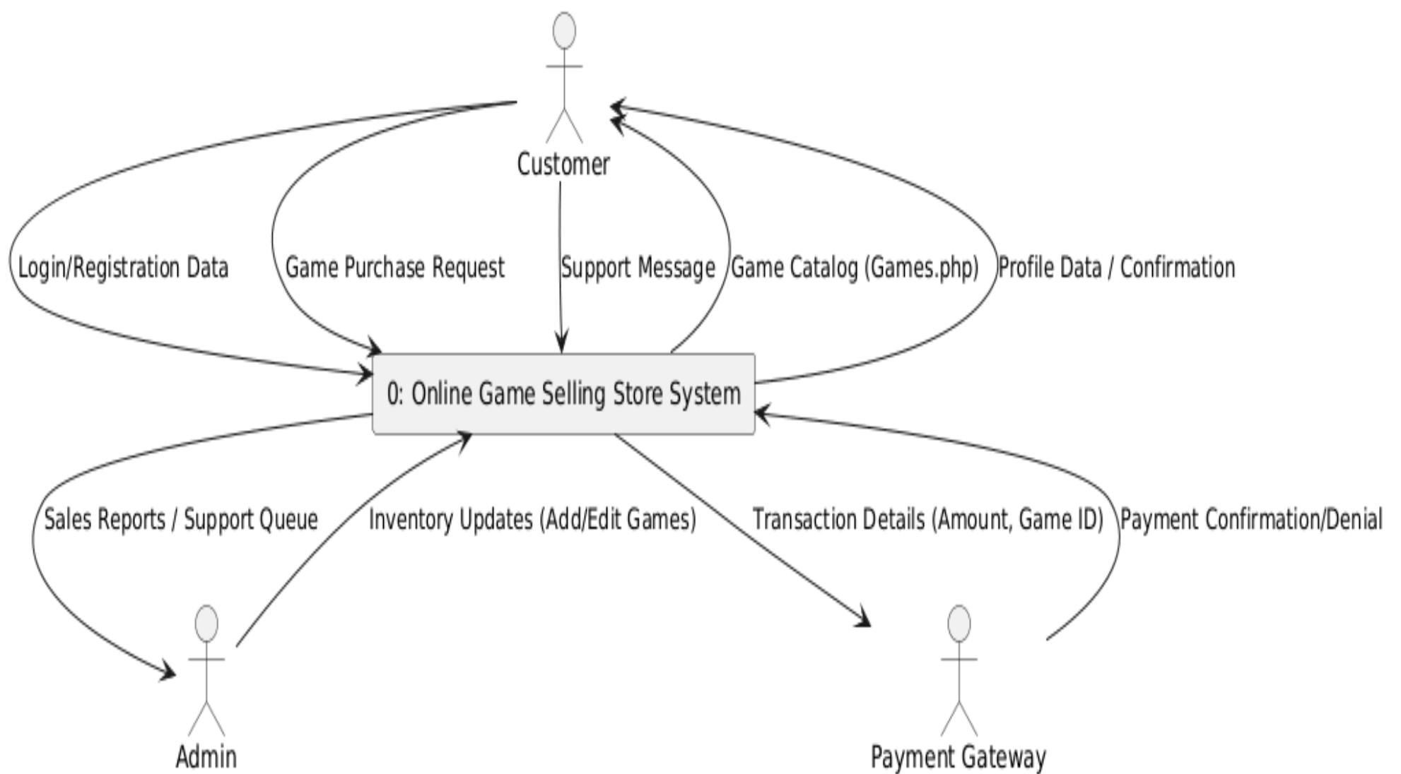
NexGenPlayz System Context Diagram
