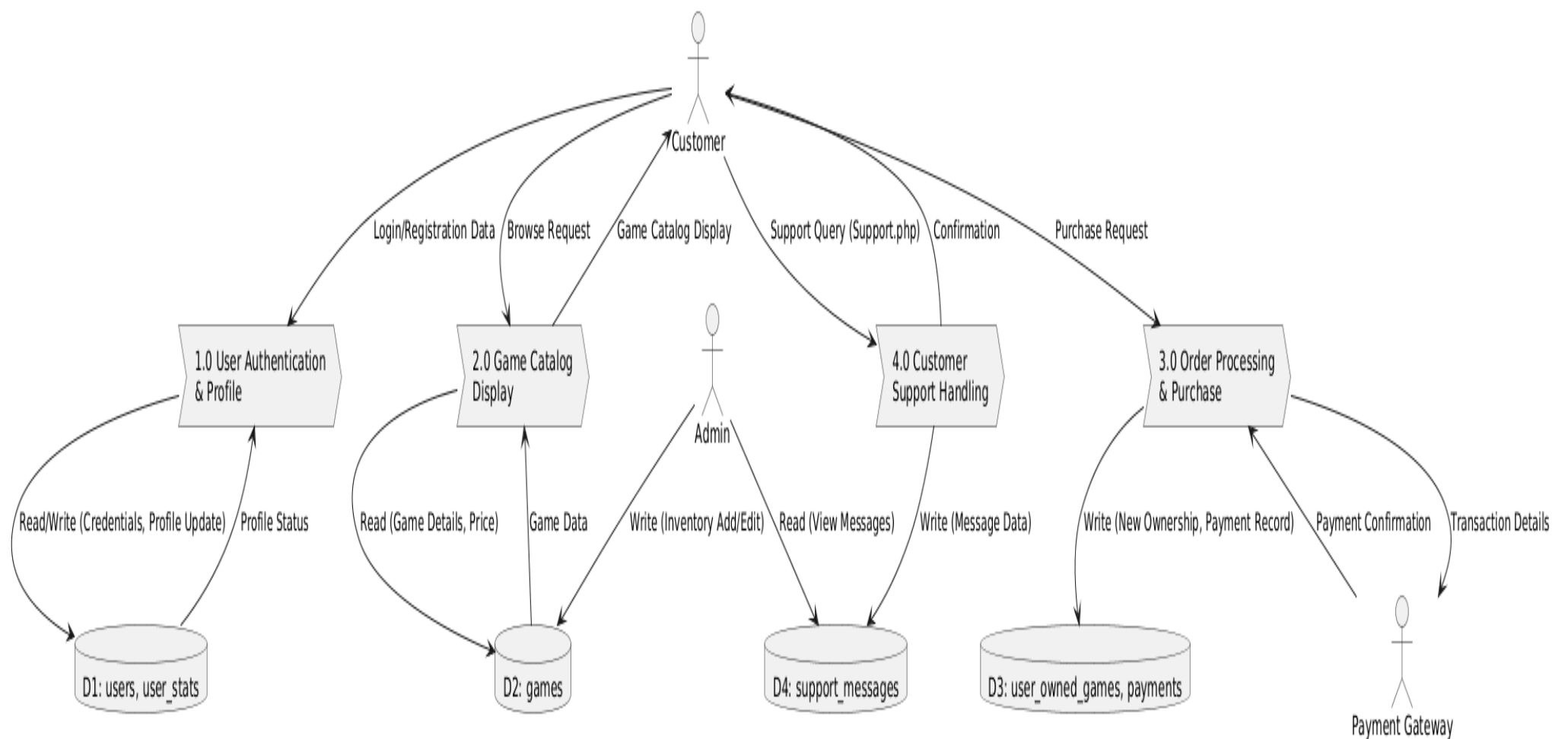
NexGenPlayz System Level 1 DFD
